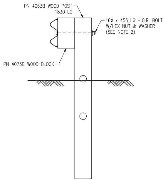
SECTION "C-C" (TYP @ POSTS #3 THRU 8)
