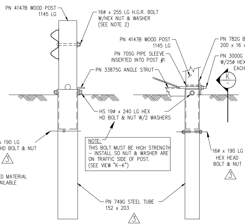
SECTION "A-A" (@ POST #2)
